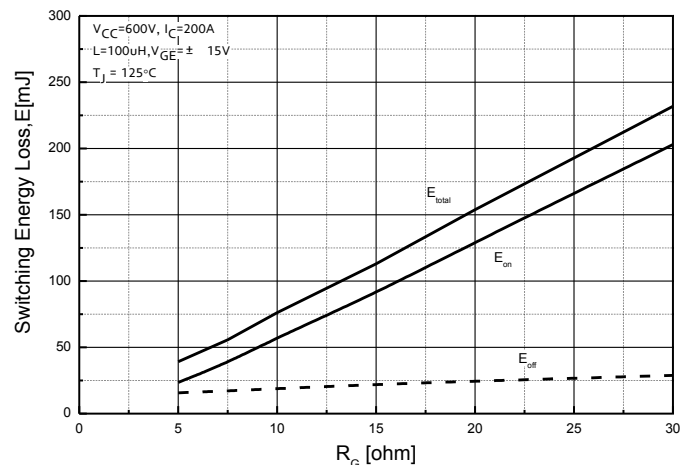
Fig. 6 Typical Switching Energy Loss = f(R_G) V_{GE} = \pm 15V, I_C = 200A, V_{CE} = 600V, T_J = 125^\circ\text{C}
